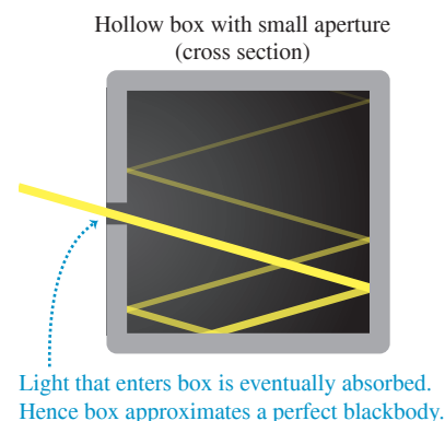
Figure 39.30 A hollow box with a small aperture behaves like a blackbody. When the box is heated, the electromagnetic radiation that emerges from the aperture has a blackbody spectrum.
